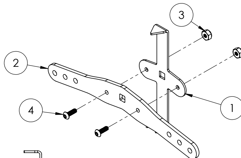
EXPLODED VIEW
